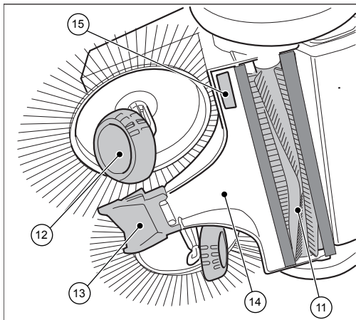
Fig. 2: Component overview 2
