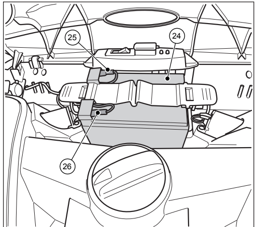
Fig. 5: Component overview 5
